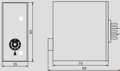
AS-DP1 Outline dimension
