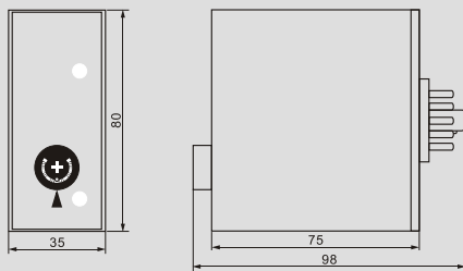
AS-DP2 Outline dimension
