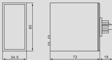
AS14S Outline dimension
